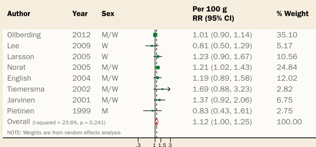
Figure 7: Dose-response meta-analysis of red meat and colorectal cancer per 100 grams per day
